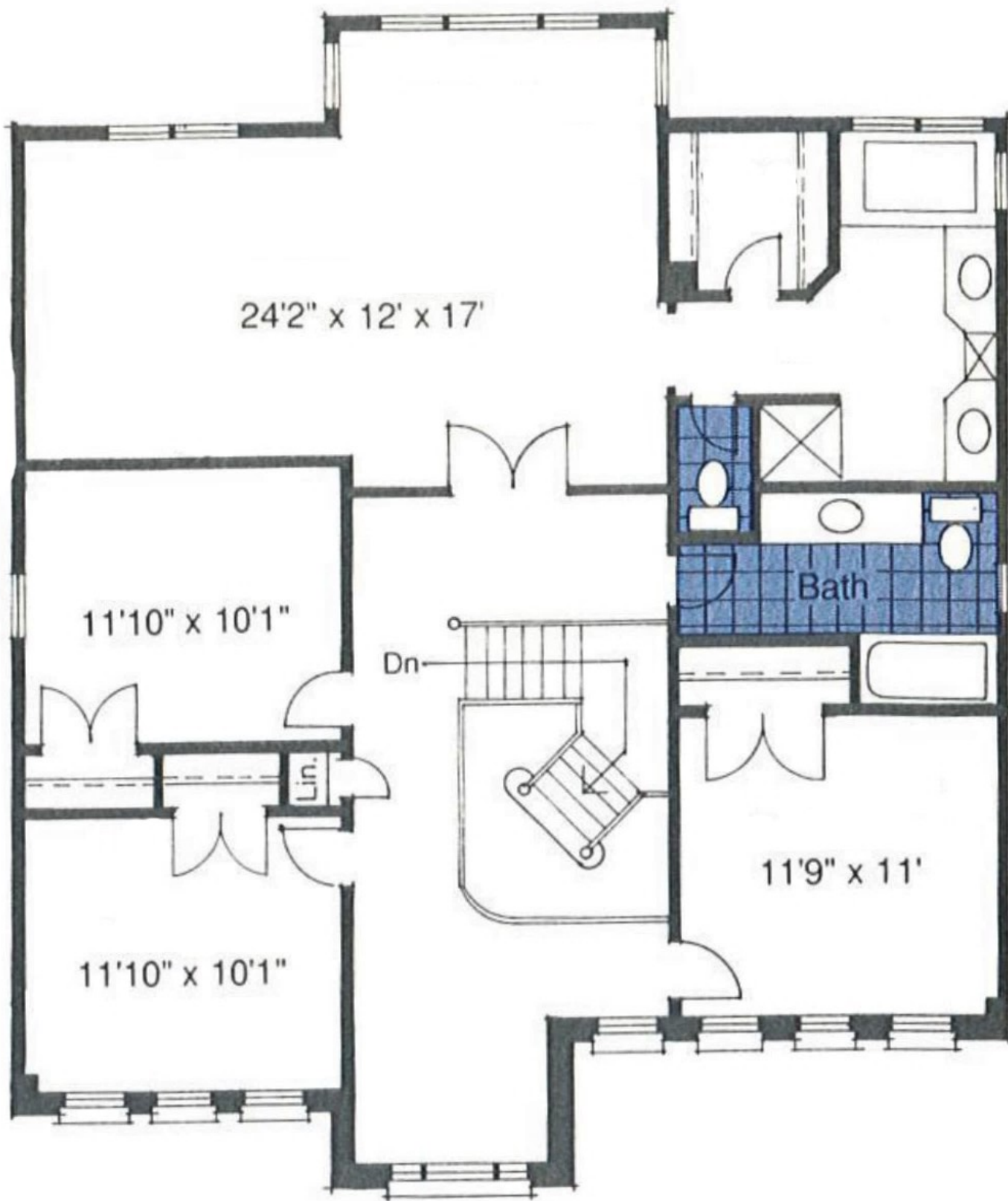
Second Floor Plan Elevation A
